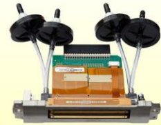
SPECTRA Polaris Print Head 35pl
